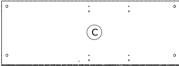
CA3447 1152x421x22mm
