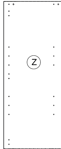
FI8389 1050x423x22mm
