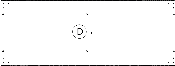
BA2113 1200x450x30mm
